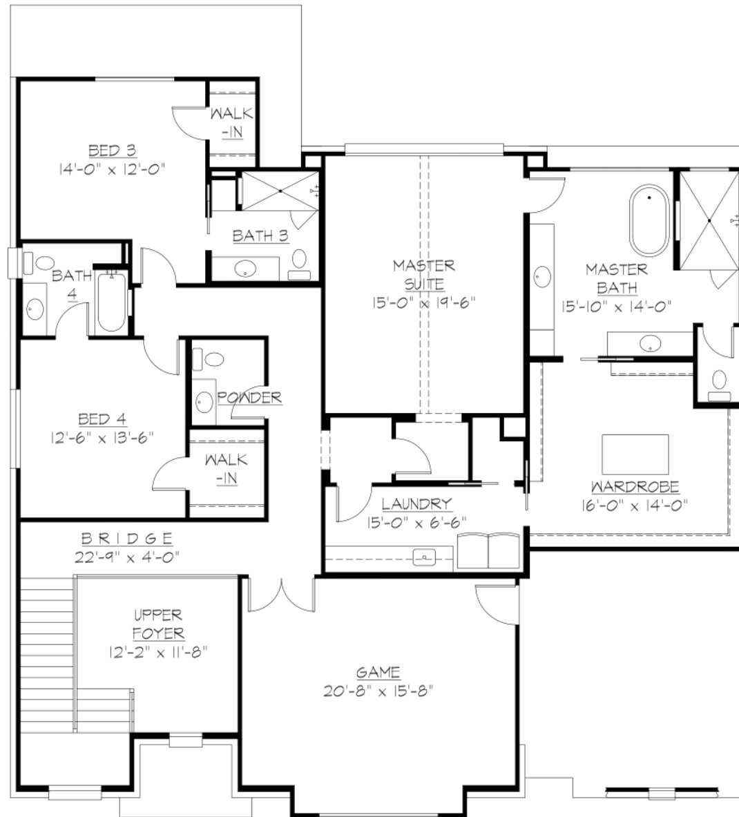
UPPER LEVEL FLOOR PLAN
