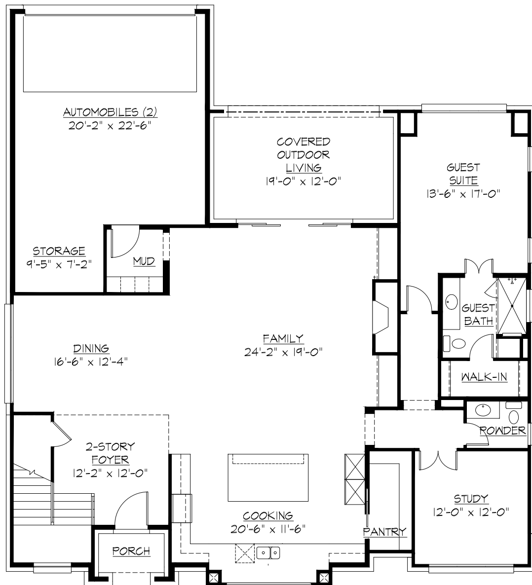
UPPER LEVEL FLOOR PLAN
